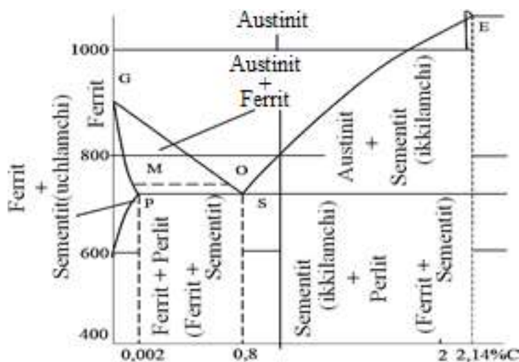
4.1-rasm. Holat diagrammaning pastki chap qismining ko'rinishi.
