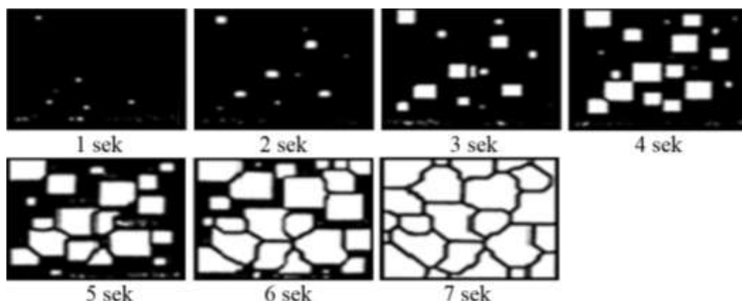
1.2-rasm. Kristallanish jarayonining modellari va kristallanish jarayonida hosil bo'layotgan kristallanish markazlaridan kristallarning o'sish holatlari.
