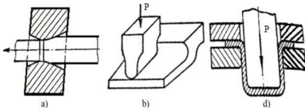
11.5-rasm. Metallarni volocheniyalash jarayoni (a), metallarga kuznets usulida ishlov berish kovkalash (b) va listli shtamplash (d) usullari.
