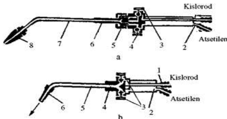
11.3-rasm. Payvandlash gorelkalari: injektorli gorelka (a) 1,2 - trubka; 3,4-ventil; 5-injektor; 6-aralashtirish kamerasi; 7-trubka; 8-mundshtuk; Injektorsiz gorelka (b): 1,2-trubka; 3-ventil; 4-aralashtirish kamerasi; 5-trubka; 6-mundshtuk tuzilishlari.
