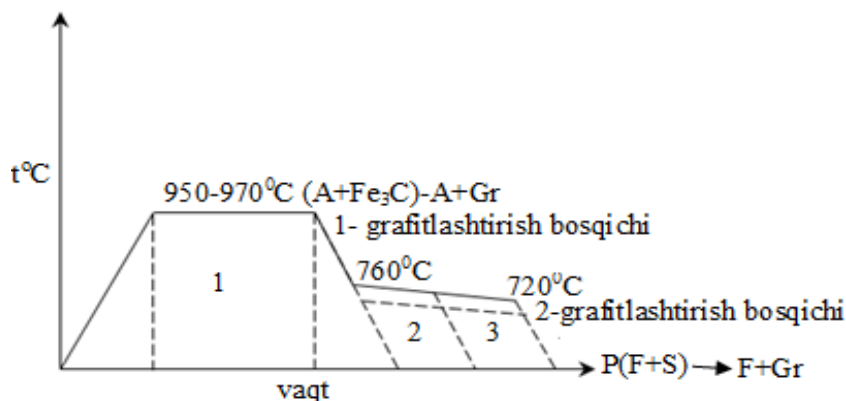
6.4-rasm. Oq cho'yanni 3 xil rejimda yumshatish grafigining ko'rinishi.
