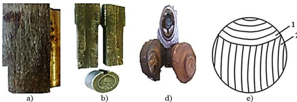
2.1-rasm. Detallarning sinish turlari: qovushqoq sinish (a); mo'rt sinish (b); toliqish oqibatida sinish (d) va toliqib sinishning sxemasi (e): 1 - darzning rivojlanish zonasi; 2 - mo'rt sinish zonasi.
