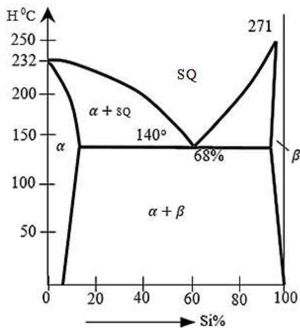
27-rasm. Sn–Bi sistemadagi qotishmalarning holat diagrammasi.
