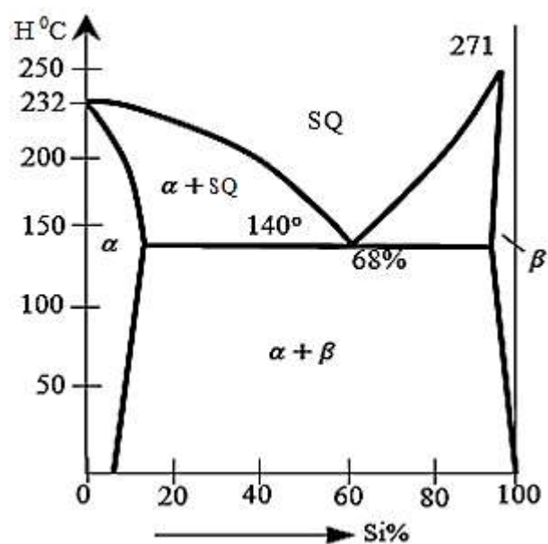
19-rasm. Sn–Bi sistemadagi qotishmalarning holat diagrammasi.
