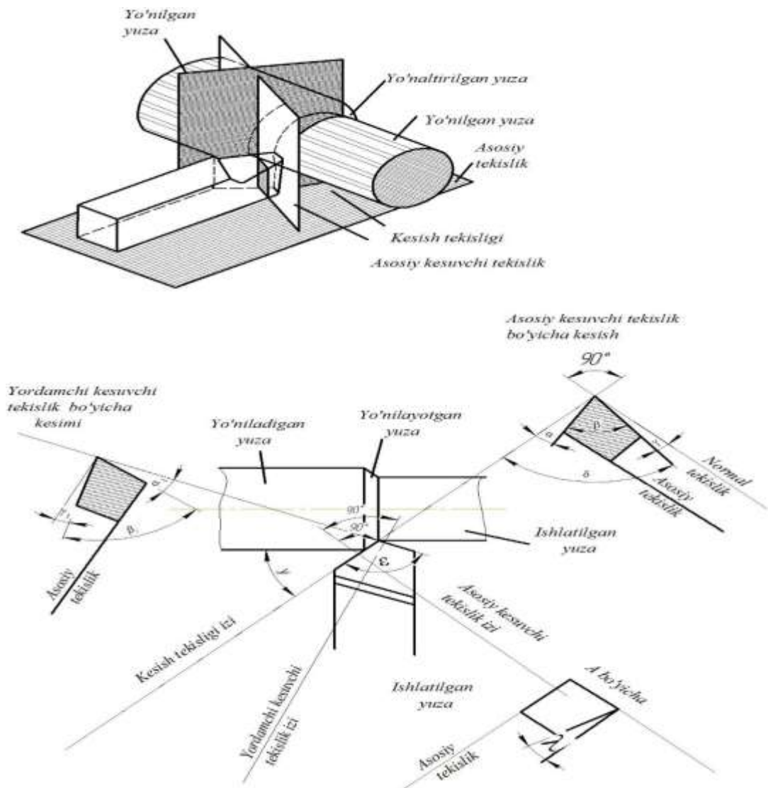
13.4-rasm. Tokarlik keskichining geometriyasi va nomlanishi.
